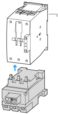
1 Contactor 2 Bases
