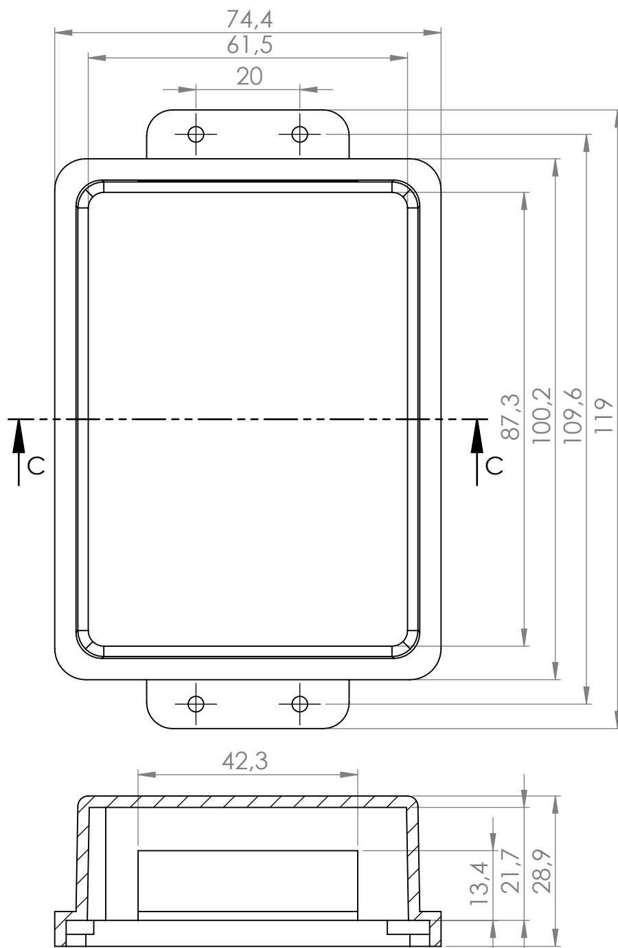
SECTION C-C
