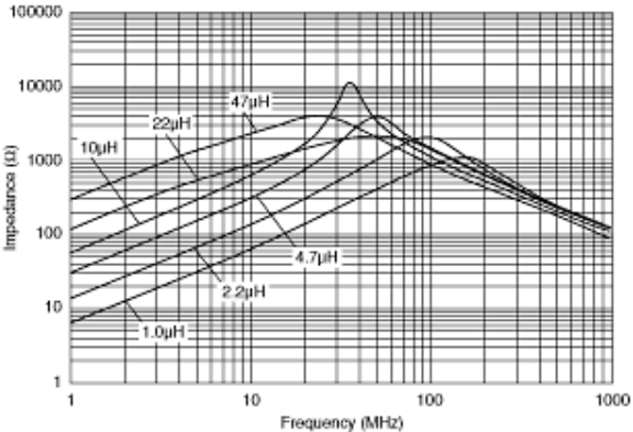
Impedance - Frequency Characteristics
