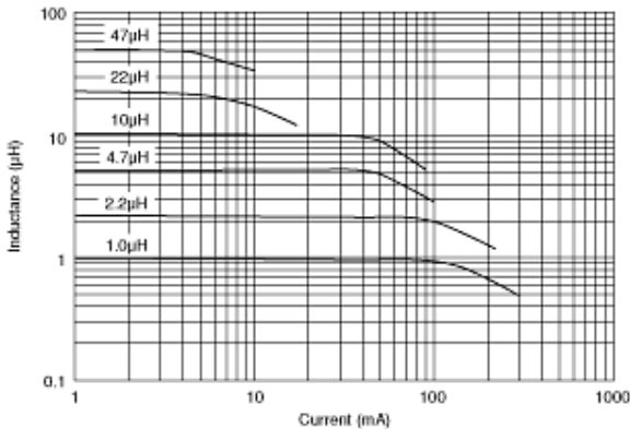
Impedance - Current Characteristics
