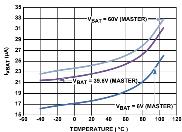
FIGURE 22B. PACK VOLTAGE SLEEP CURRENT vs TEMPERATURE AT 6V, 39.6V, 60V (DAISY CHAIN MODE)
