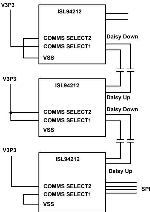
FIGURE 32. DAISY CHAIN COMMUNICATIONS CONNECTIONS AND SELECTION
