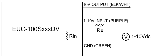
Implementation 3: External resistor and 1-10V DC Input
