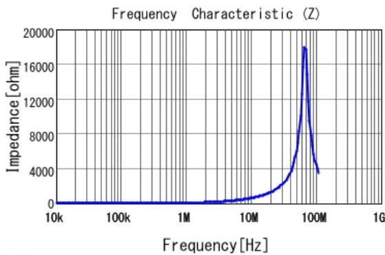
■ LQH2MCN100K02 |Z|
