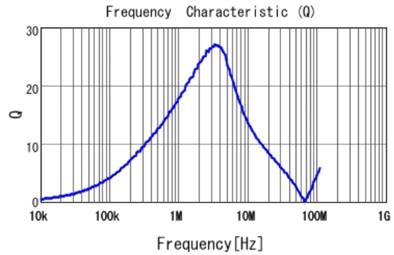
■ LQH2MCN100K02 Q
