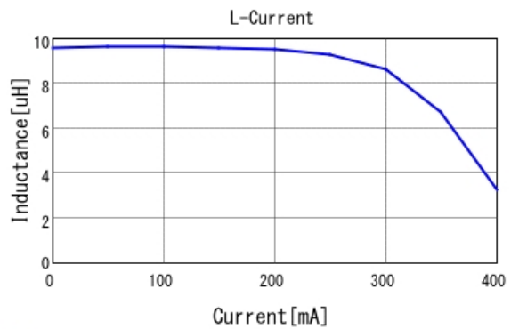
■ LQH2MCN100K02 L-Current 20degC
