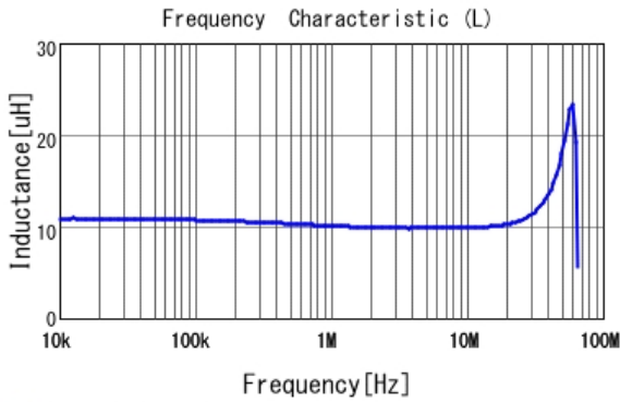
■ LQH2MCN100K02 L
