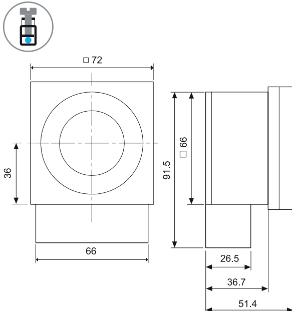
12.31 Screw terminal
