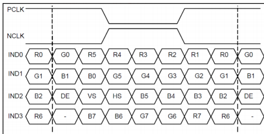
Figure 5. 8-bit LVDS Input Timing chart
