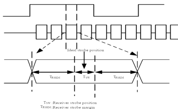
LVDS timing(2)
