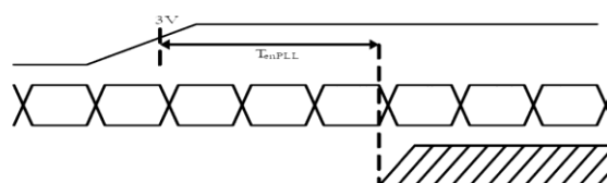
LVDS timing(2)
