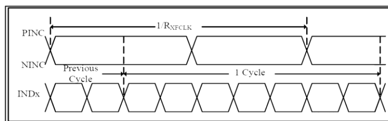
LVDS timing(1)
