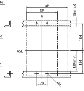
Drilling plan (front view)
