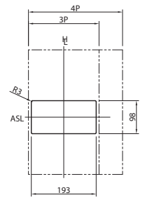
Panel cutout (front view)
