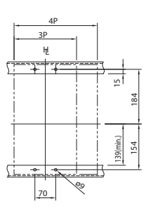
Drilling plan (front view)
