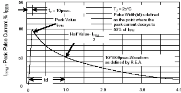
Fig.3 - Pulse Waveform
