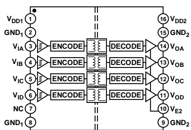
Figure 1. ADuM1400
