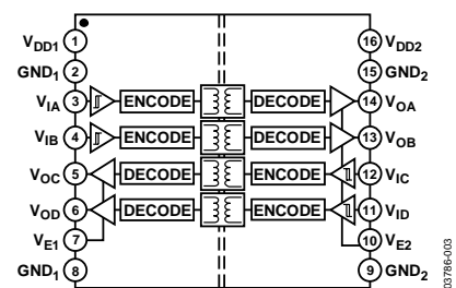
Figure 3. ADuM1402
