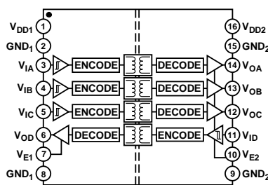
Figure 2. ADuM1401
