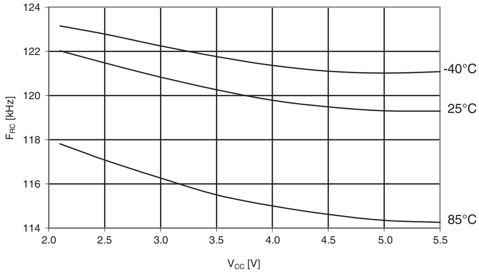
Figure 30-332. Atmel ATmega1284: Watchdog oscillator frequency vs. V CC .
