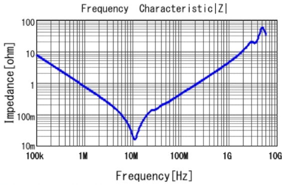
■ GRM43DR72E224KW01 |Z| DCOV, 25degC
