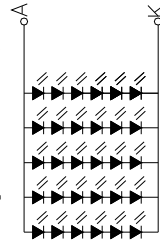
Circuit Diagram(LED SMT 6*5=30 PCS), Color: WHITE
