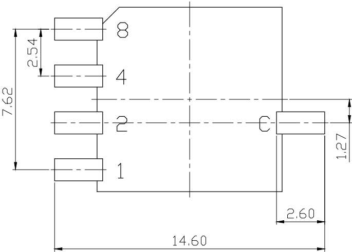
P.C.B DIMENSION (TOP VIEW)
