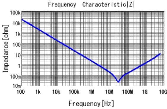
■ GRM155R61A104KA01 |Z| DCOV, 25degC
